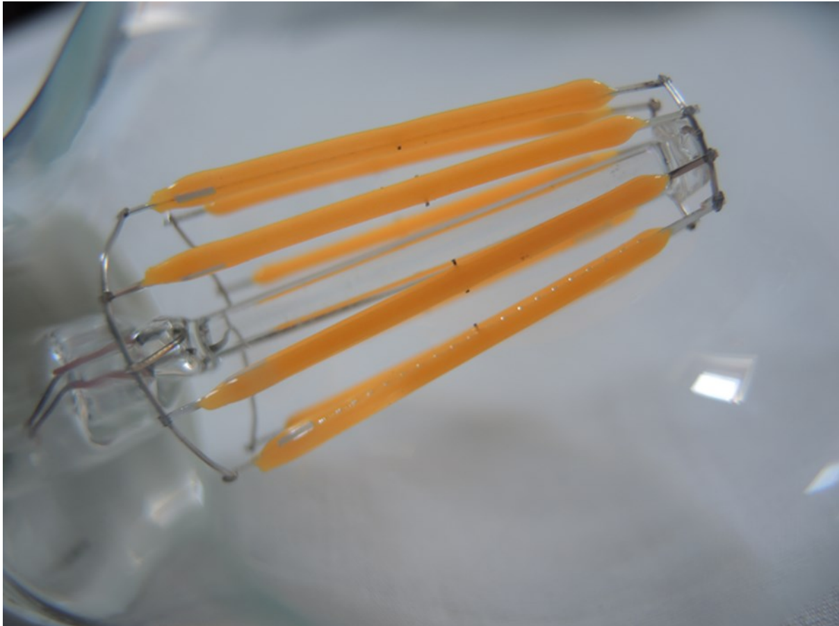
Figure 2-4. Close-up photograph of LED filaments from LED Connection (UK) 8W lamp
