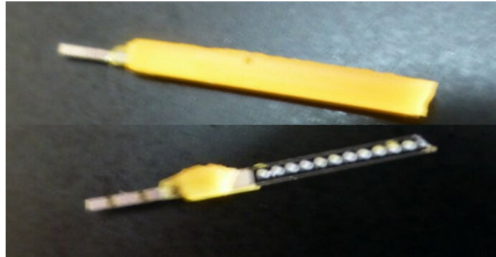
Figure 2-5. Cut-away view of LED filament on transparent substrate
