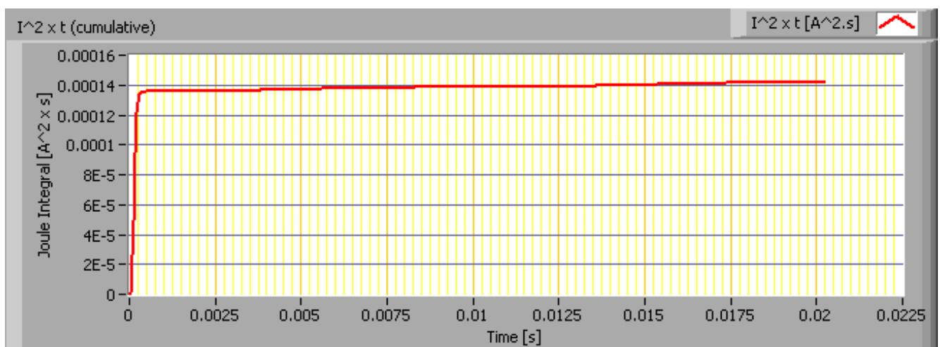
The value I^2 \cdot \Delta t for the first 10 ms.
