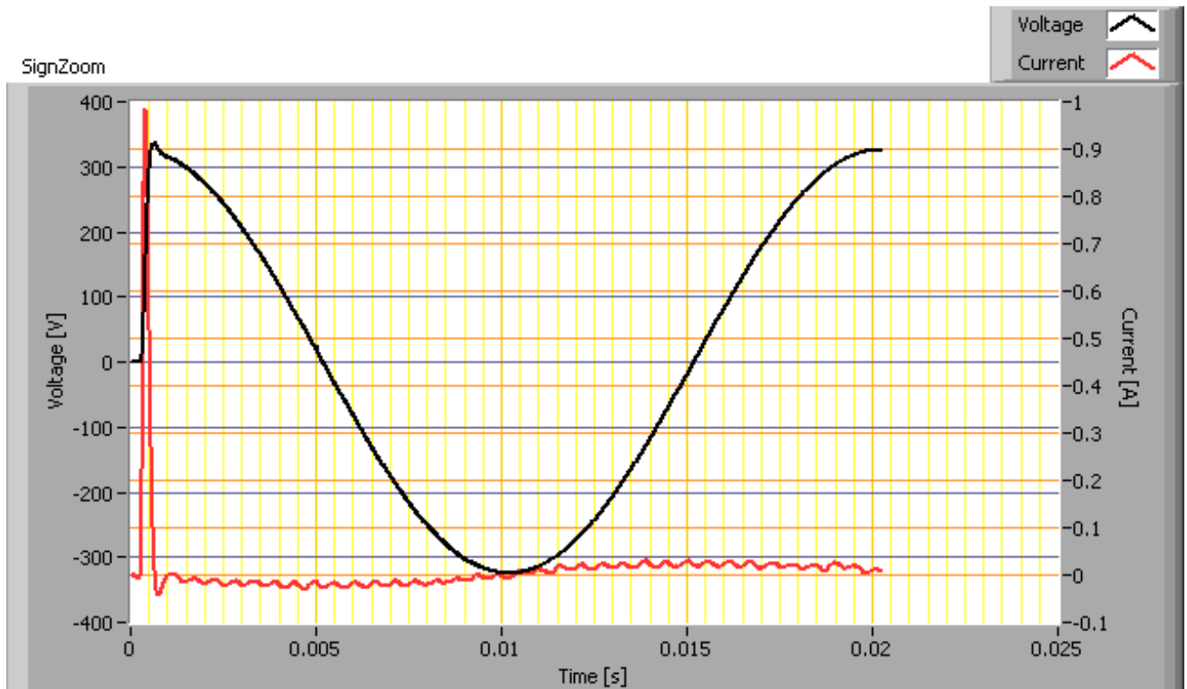
First cycle of worst case inrush current.
