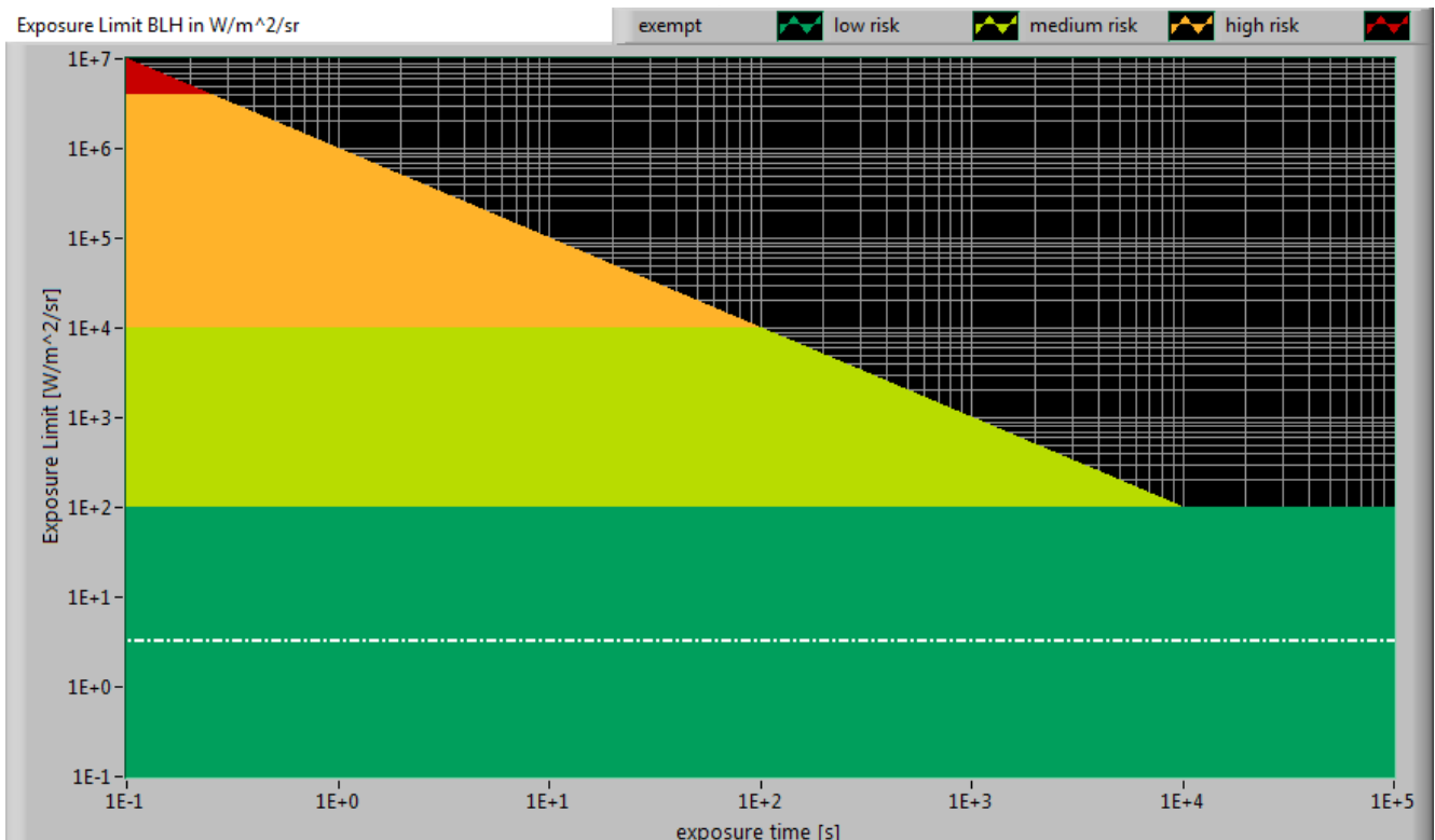
The level of blue light of this lamp related to the exposure limit and the different classification areas.
