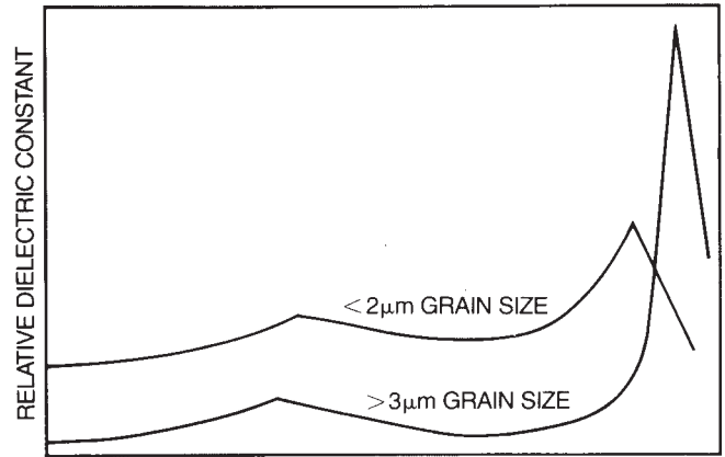
Figure 3. Small-signal dielectric constant varies with temperature
